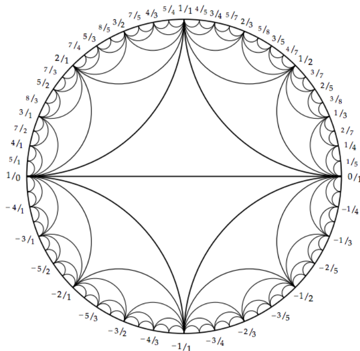
FIGURE 2. Farey diagram.
